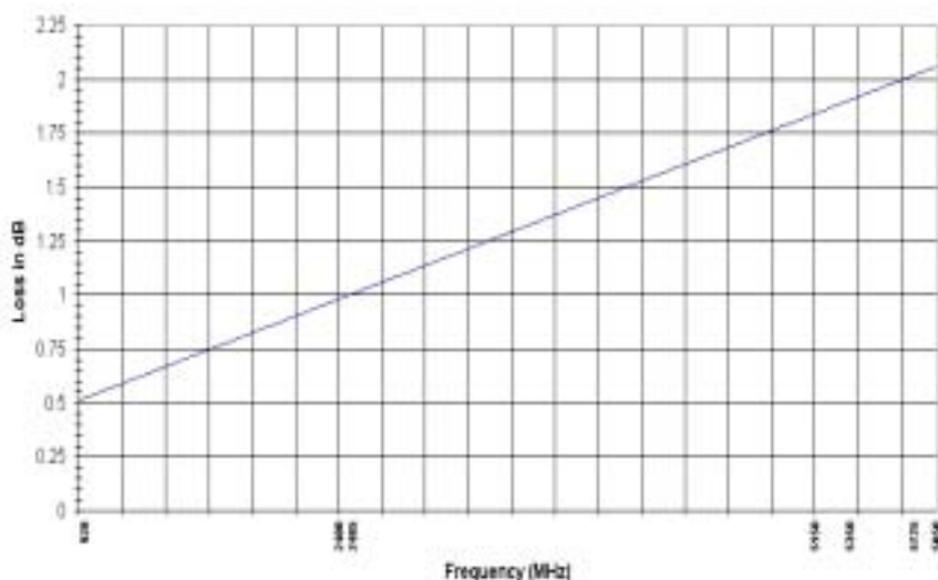
MR-RD Loss Versus Frequency
